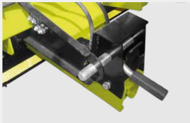
EASY TO BE OPERATED, SAFE LOCKING With large tolerances when loading and unloading the header
